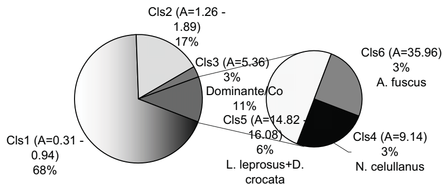
Fig. 4. – The relative abundance of 35 species of Aranea from Cheile Carașului transposed on an estimated scale of 6 classes.
